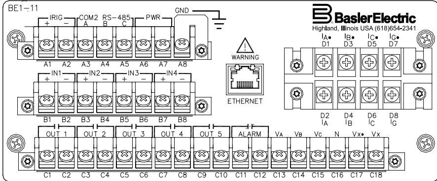
Figure 8 - BE1-11g H- and P-Case Style Rear Panel Connections
