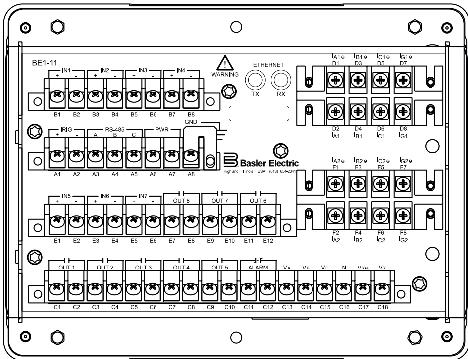
Figure 9 - BE1-11g J-Case Style Rear Panel Connections
