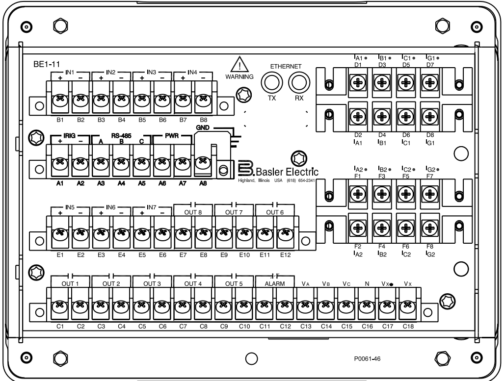
Figure 6 - J Case Rear Panel Connections (shown with optional Fiber optic Ethernet port)
