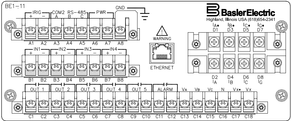
Figure 6 - BE1-11f H- and P-Case Style Rear Panel Connections
