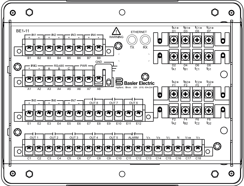
Figure 7 - BE1-11f J-Case Style Rear Panel Connections
