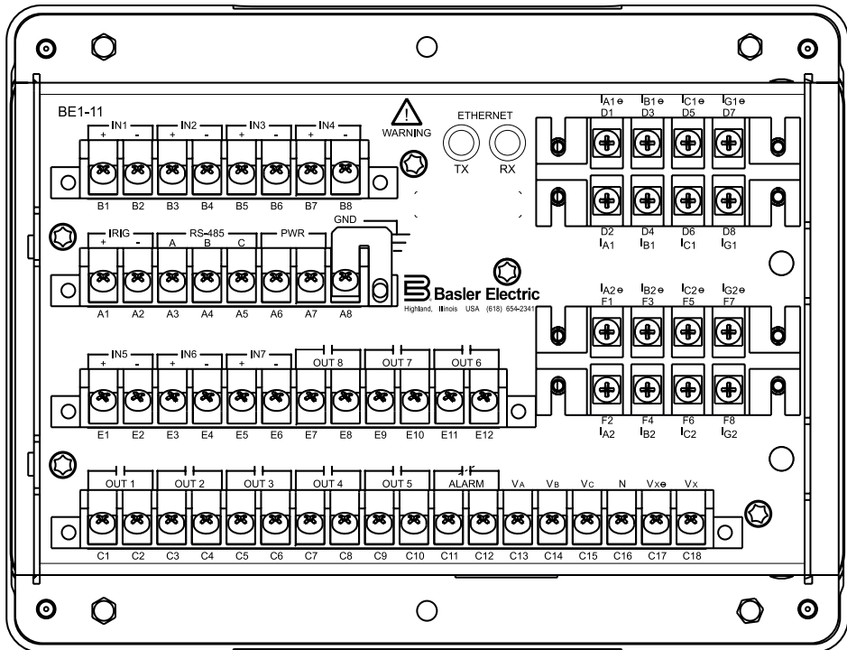
Figure 7 - BE1-11i J-Case Style Rear Panel Connections
