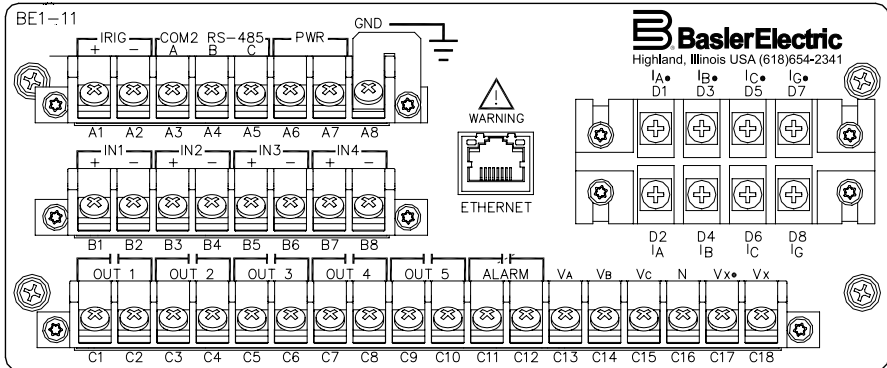
Figure 6 - BE1-11i H- and P-Case Style Rear Panel Connections
