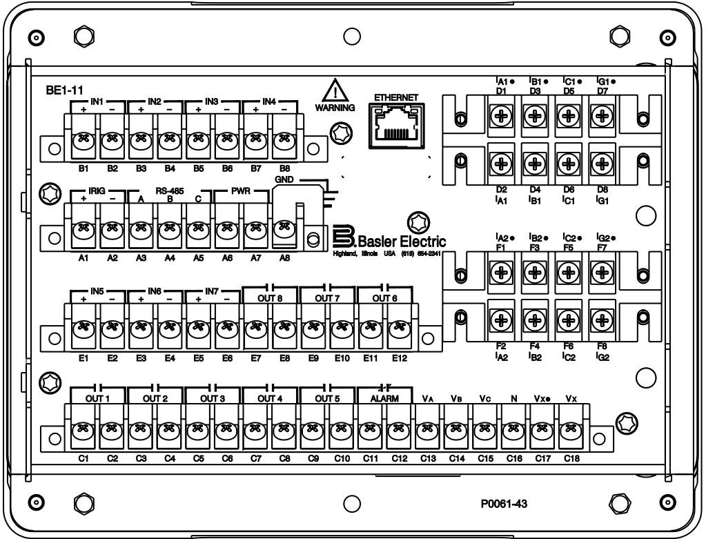
Figure 5 - J Case Rear Panel Connections (shown with optional RJ45 Ethernet port)
