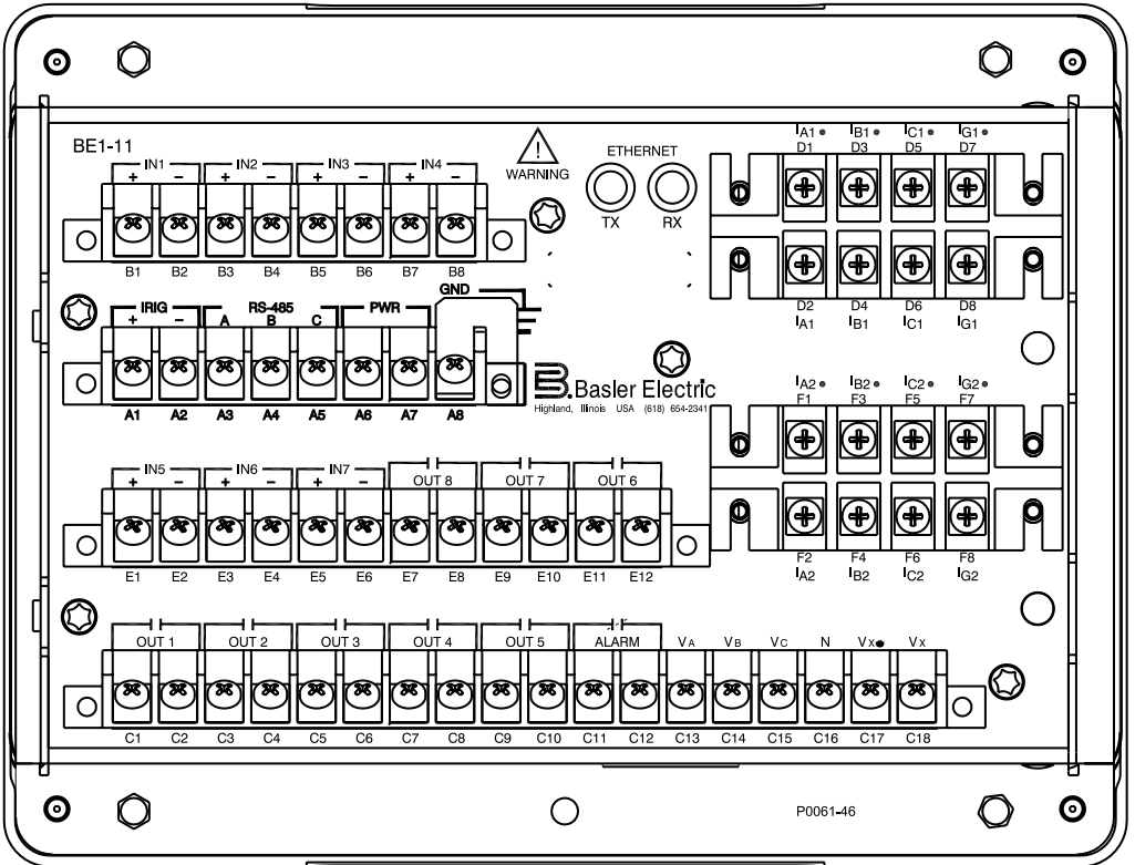
Figure 6 - J Case Rear Panel Connections (shown with optional Fiber optic Ethernet port)
