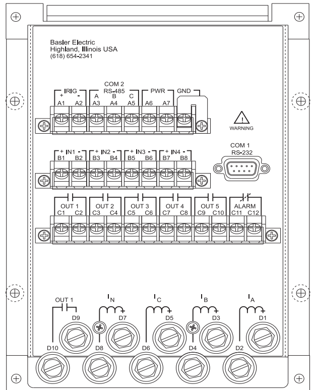
Figure 5C - BE1-851 S1 Rear Panel Connections
