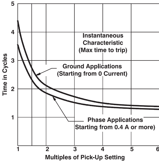
Figure 2 - Instantaneous Characteristics
