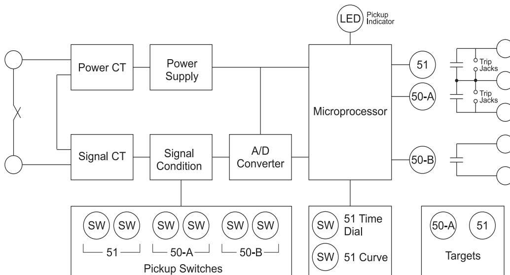
Figure 1 - Functional Block Diagram - Models with 2 Instantaneous
